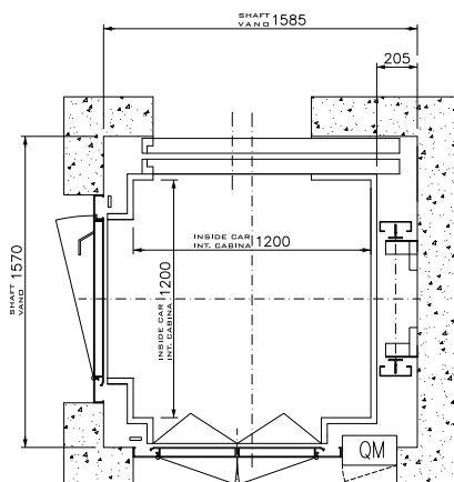
VANO IN MURATURA SHAFT WALLING
